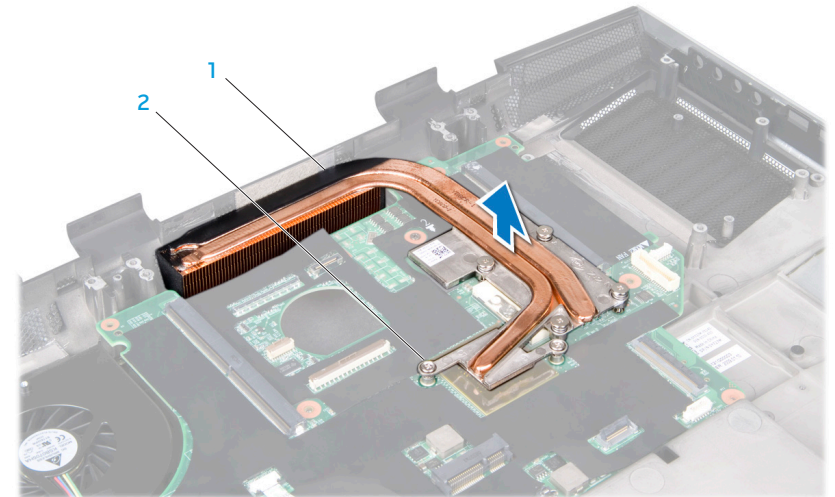
1 processor heat sink
